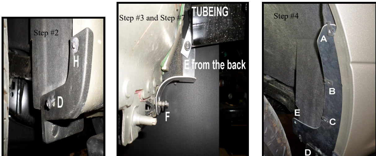
FF12 15 150 NF, FF12L 15 150 2- Aluminum (AL) Flat Clips #10001 ; 2-(AL) F150 Brackets #10053
